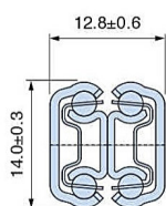
Cross sections
