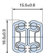
Cross sections
