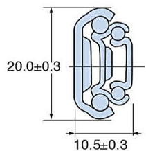
Cross sections
